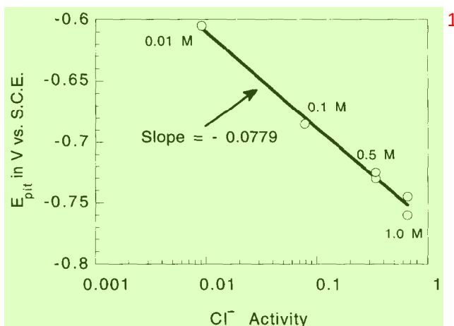
Fig. 1. Pitting potentials for aluminum as a function of chloride ion activity.
