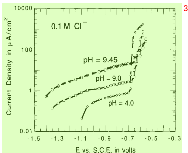
Fig. 4. Anodic polarization curves for aluminum in 0.1 M NaCl at three different pH values. 4
