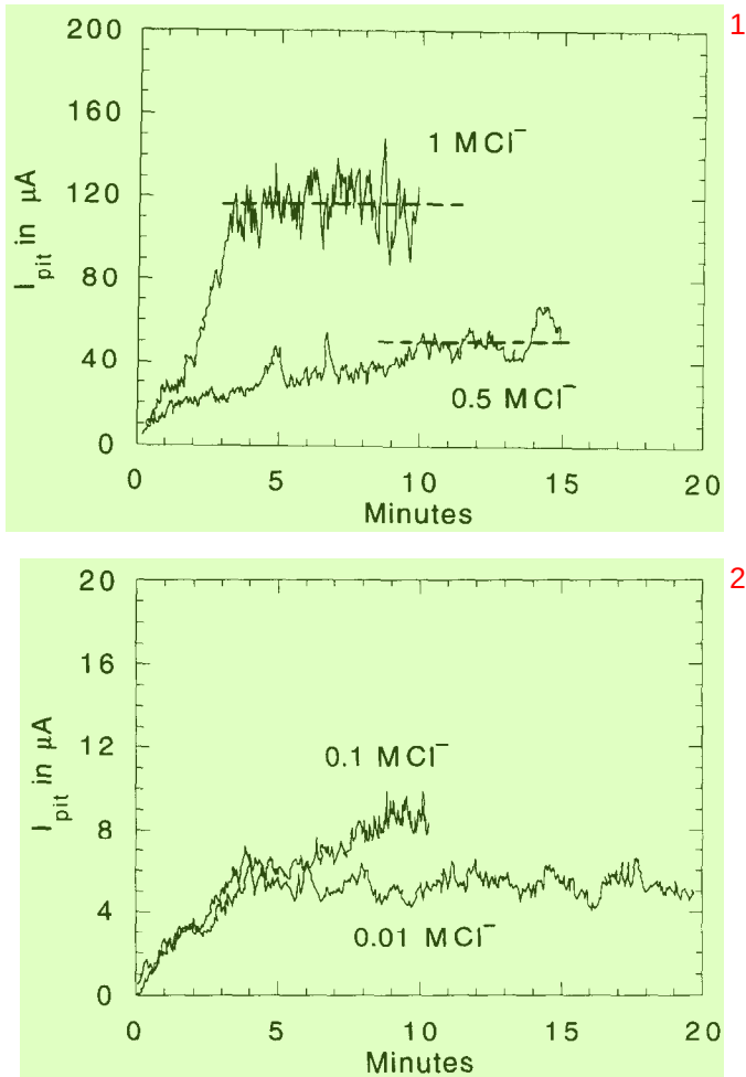
Fig. 2. Pitting current for aluminum in various chloride solutions (at the pitting potential in each case).
