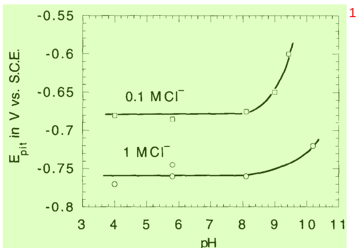
Fig. 3. Pitting potentials for aluminum as a function of pH in 0.1 and 1 M chloride solutions. 2
